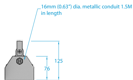
End view - conduit exit side
